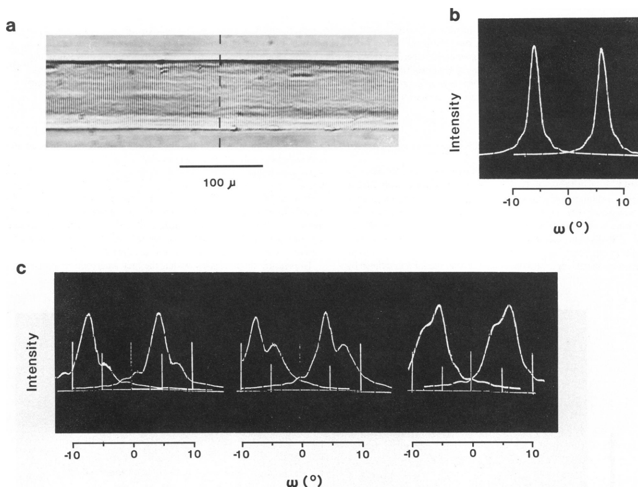
FIGURE 3 Effect of beam incidence angle \omega on the total intensity of the first order diffraction maximum ( \omega -scan). (a) Micrograph of an exceptionally regular fiber segment. The laser beam is oriented as indicated by the dashed line. Sarcomere length was systematically measured at 70 points within this micrograph. At each point sarcomere length was calculated from the total length of 20 sarcomeres in series. Sarcomere length varied between 2.34 and 2.42 \mu\text{m} with an average of 2.38 \pm 0.02 \mu\text{m} (SD). Reading accuracy, 0.01 \mu\text{m} . Fiber diameter (from micrograph), 85 \mu\text{m} . Note, the fiber region shown represents the area that was illuminated by the laser beam when \omega -scans of b were recorded. (b) \omega -scans of left- and right-hand first-order diffraction maxima of the same fiber segment shown in a. Abscissa, angle \omega ; ordinate, intensity in the first-order diffraction maximum. Beam diameter, 0.5 mm. Note the very narrow range over which significant intensity is detectable in the first orders. This is found only when the striation pattern is as regular as it is in a. At perpendicular beam incidence ( \omega = 0 ), the intensity in either first-order maximum is only about 1/20 of the maximum observed when the incidence angle is about \pm 6^\circ . (c) Three typical \omega -scans of single skinned rabbit psoas fibers with somewhat less regular striation patterns. Coordinates same as in b. Note the almost identical shape and amplitude of the two \omega -scans in all cases. Each pair appears to be composed of almost identical maxima separated by about the same angle. To demonstrate the high reproducibility of these \omega -scans, all records were traced several times (traces superimposed).
