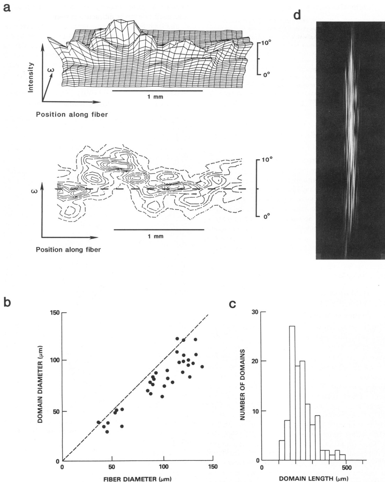
FIGURE 5 Size and number of domains within a fiber segment, determined from \omega -scans, vs. substructural lines within the first-order diffraction line. (a) Display of a series of \omega -scans along a fiber segment as a three-dimensional map (top) and as a corresponding intensity contour map (bottom). \omega -scans were recorded every 60 \mu\text{m} . Total segment length represented by this series is \sim 2 mm. Beam diameter \sim 60 \mu\text{m} . Note the length along the fiber and the narrow range of incidence angles for which a single peak of intensity can be followed. Taking each individual peak as the contribution of a single domain, about 15 domains can be identified. At the incidence angle, which is indicated by the dashed line in the contour map, at most five domains will contribute to the diffraction pattern of the 2-mm segment. (b) Diameter of domains estimated from the FWHM of the intensity peaks in \omega -scans vs. fiber diameter. For details of calculation see second part of the Appendix. The
