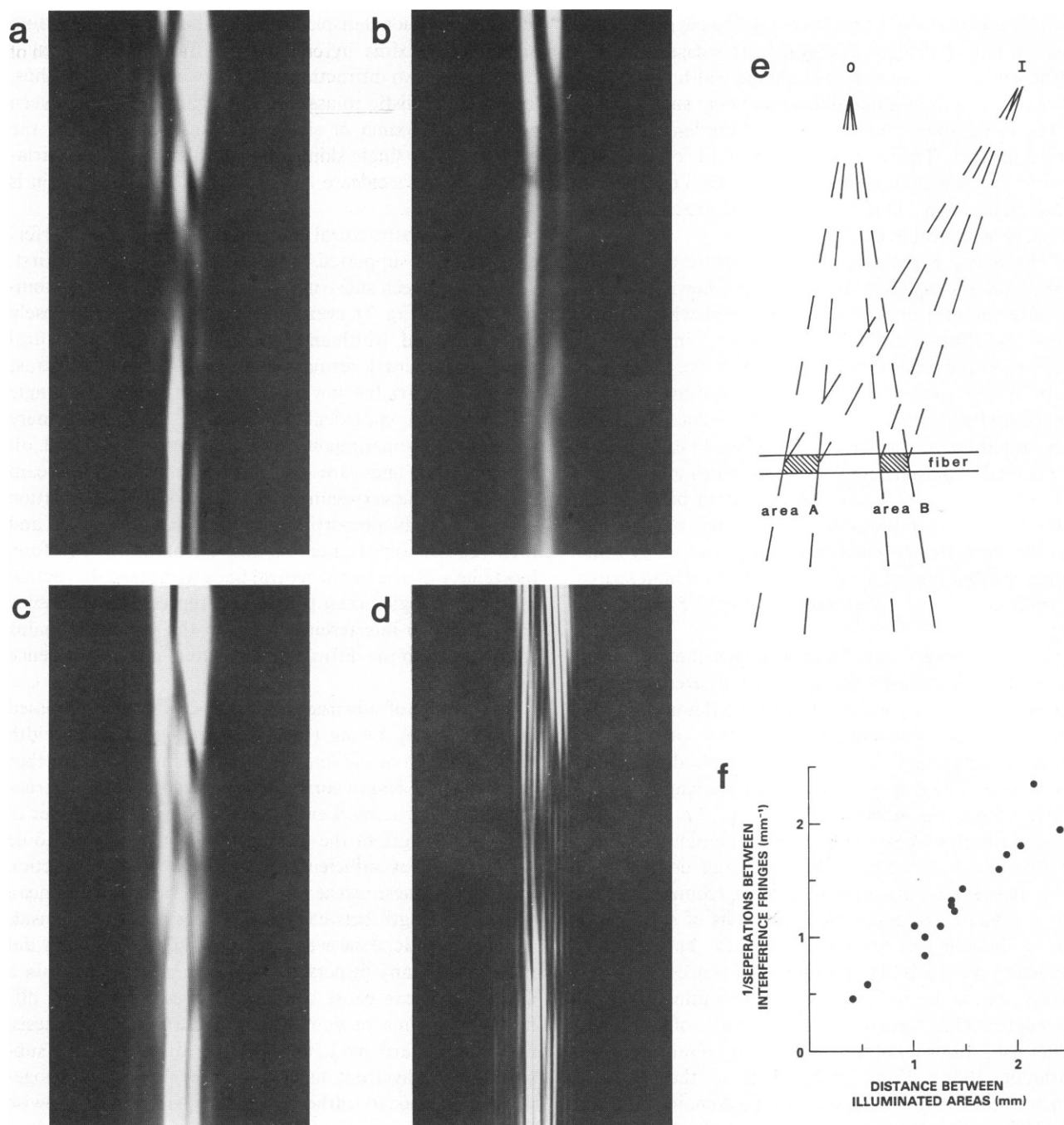
FIGURE 8 Double-beam experiment. Effect of simultaneous illumination of two fiber areas, A and B , within a fiber. (a) First-order diffraction maximum observed when only area A is illuminated. (b) First-order diffraction maximum observed when only area B is illuminated. (c) Sum of first-order diffraction maxima of A and B , obtained by superposition of the two films shown in a and b . (d) First-order diffraction maximum observed when A and B are illuminated simultaneously. Note, that here the "underlying" intensity distribution is similar to c , but there is also "line splitting" as the result of interference between A and B . (e) Schematic drawing on the optical arrangement. Note, the two beams are arranged such that their foci superimpose in the film plane. This is achieved by either the beam-splitter/mirror system (Fig. 1) or by placing a double slit in the path of an expanded beam focused onto the film plane. (f) Effect of center-center distance between the two illuminated areas on the width of the additional lines (interference fringes), observed when both areas were illuminated simultaneously ( d ).
